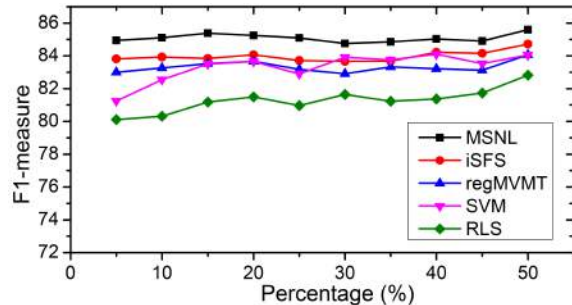
Figure 4: F1-measure at different fraction of volunteer samples.
